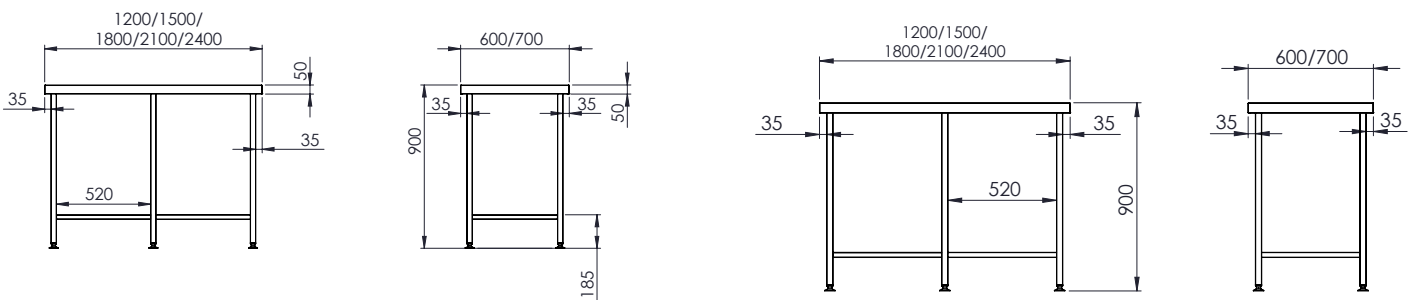
Stainless Steel Table with Part Undershelf (left side) - Page 72
