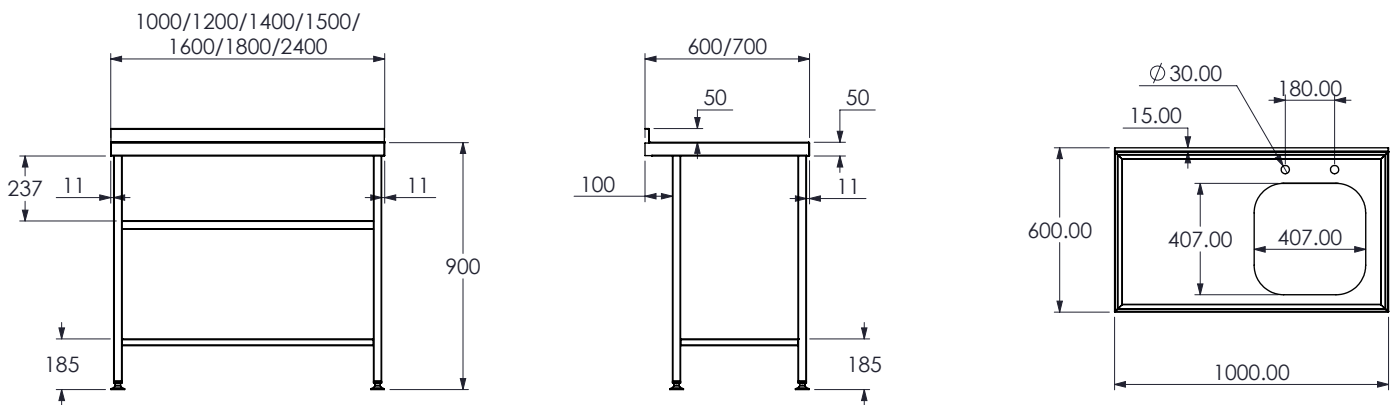
Stainless Steel Fully Assembled Sink - Page 62
