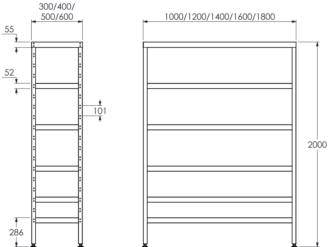
Stainless Steel Storage Racks with 6 Shelves and Adjustable Feet - Page 81
