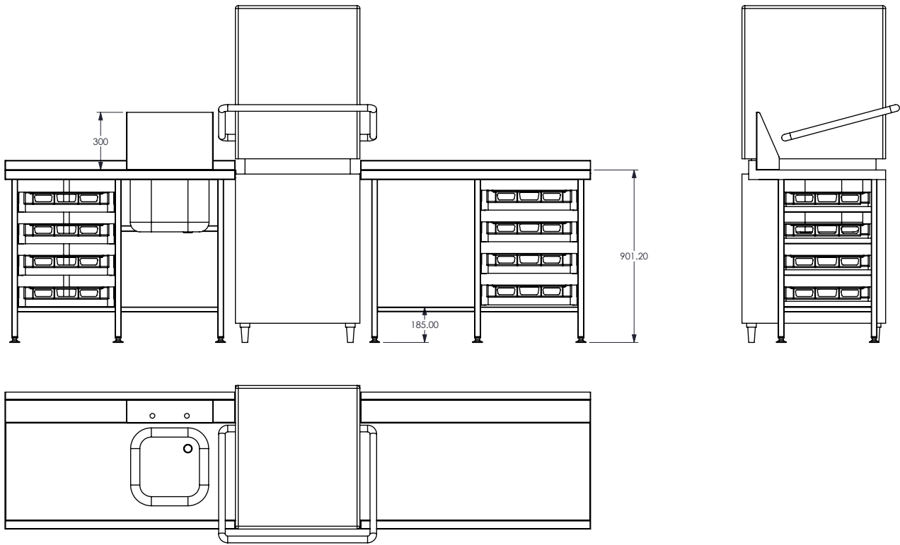
Dishwasher Tables - Page 60
